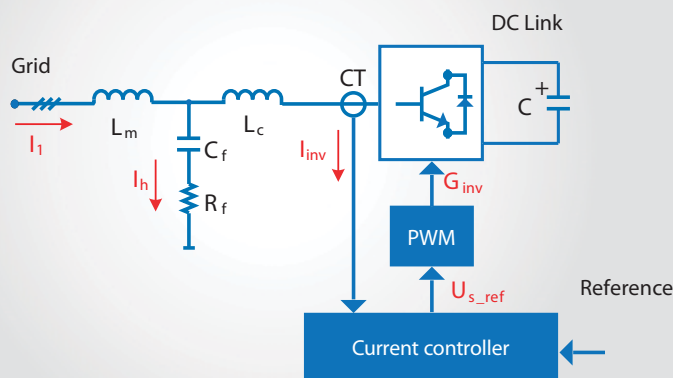
Traditional Active filter control
