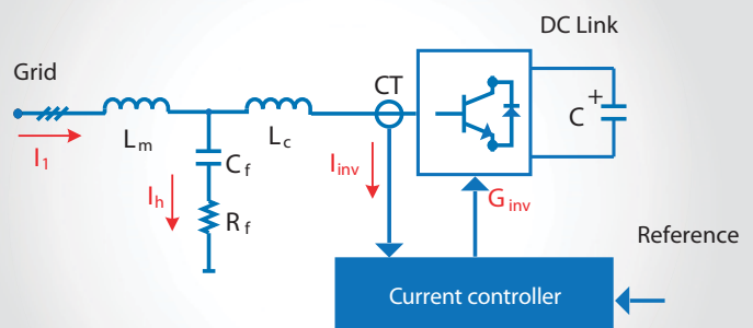
VLT® Active Filter control
